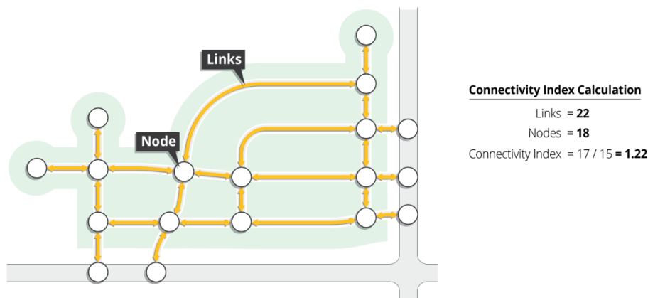
Figure 8.1: Connectivity Index Calculation
