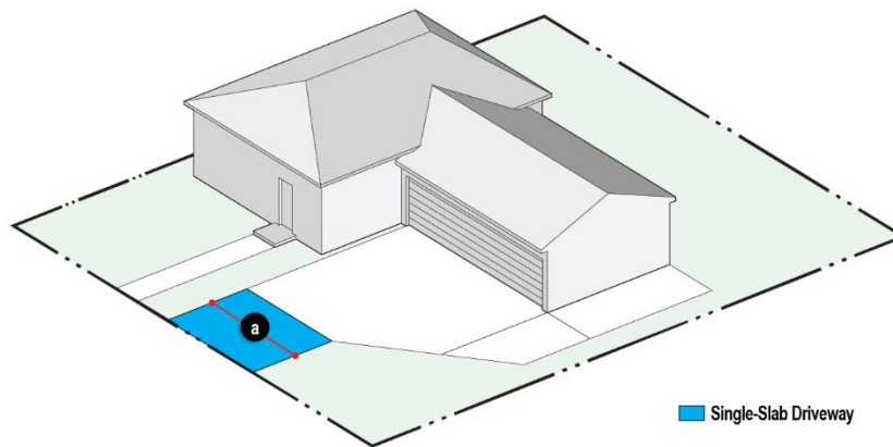
Figure 6.4: Single-Slab Driveway Design Standards
