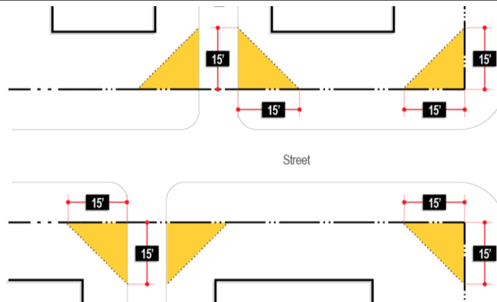
Figure 6.29: Visibility Standards Fence A
