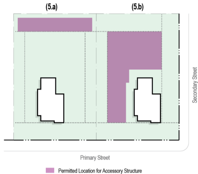
Figure 5.7: Accessory Structures Permitted Locations
