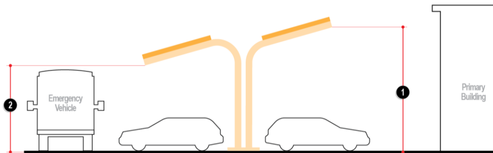
Figure 5.9: Canopy Solar Energy Collection Systems
