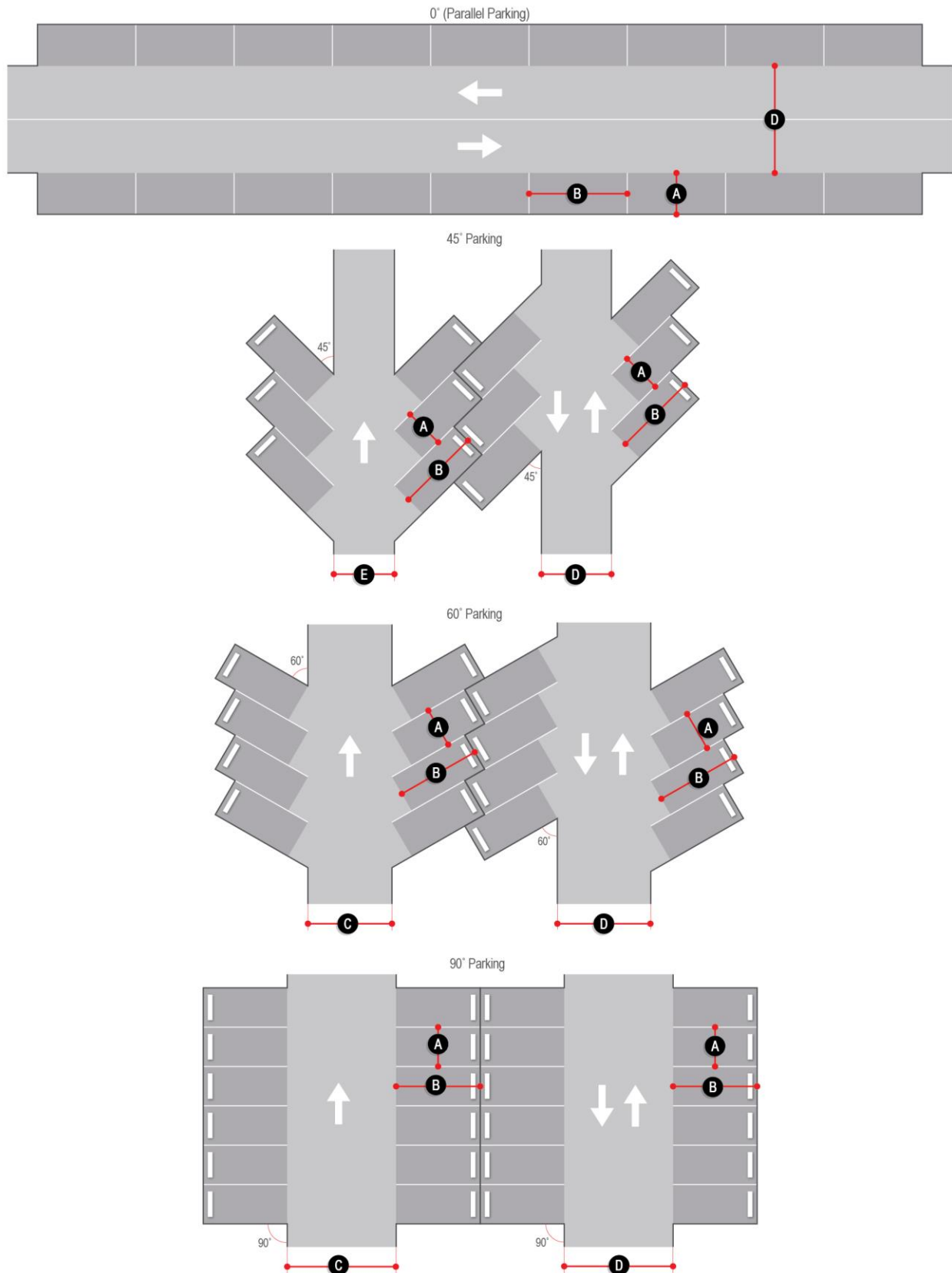
Figure 6.1: Dimensional Requirements of Parking Spaces and Maneuvering Lanes
