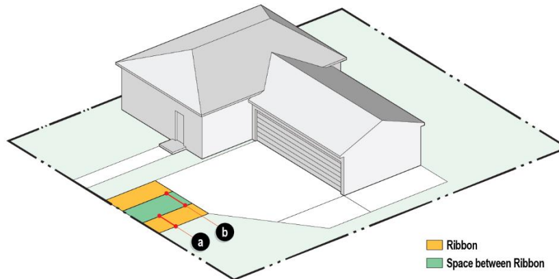
Figure 6.5: Ribbon Driveway Design Standards
