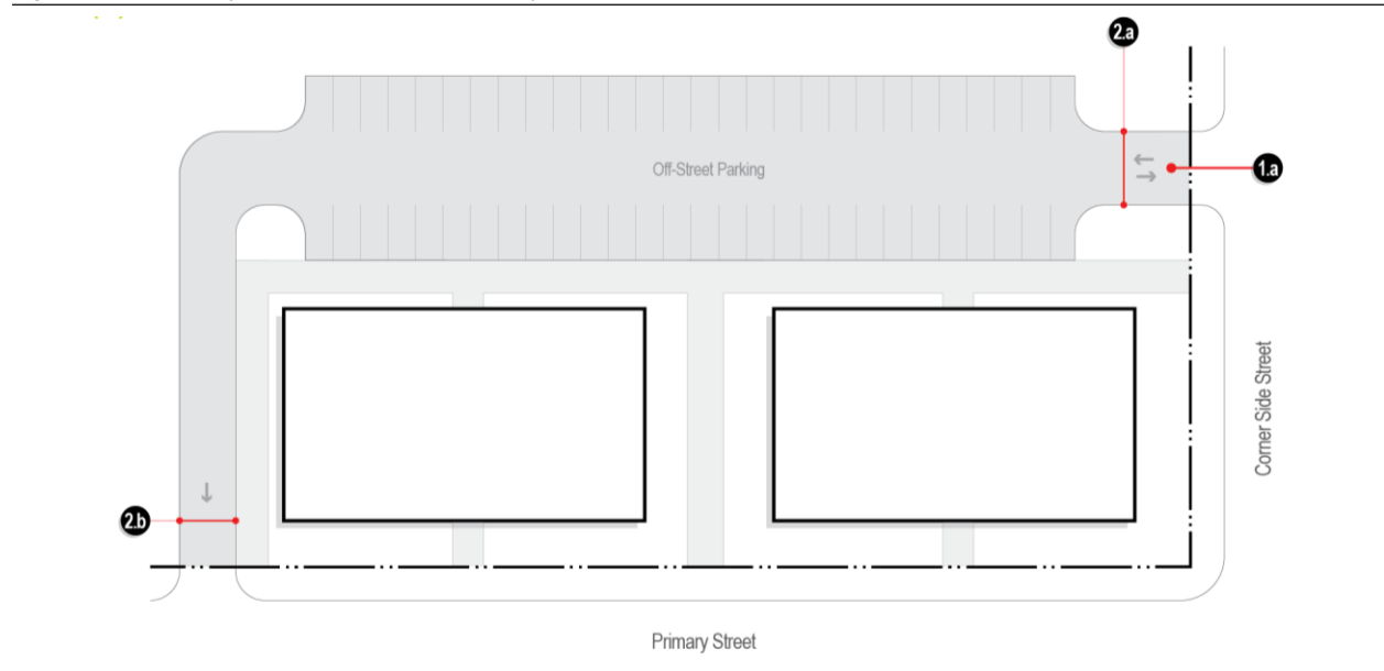
Figure 6.8: Multifamily and Nonresidential Driveway Standards
